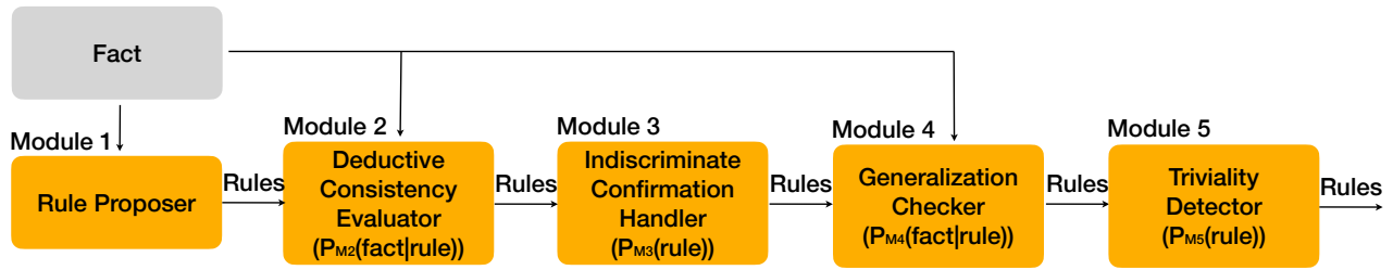
Figure 1: Our proposed framework (CoLM) for inductive reasoning with natural language representation task. Rule Proposer is a generative model based on input facts and desired rule template, aiming at generating (a large number of) rule candidates. Deductive consistency evaluator, indiscriminate confirmation handler, generalization checker, and triviality detector are classification models that filter improper rules according to four requirements of the induced rules in inductive reasoning.
