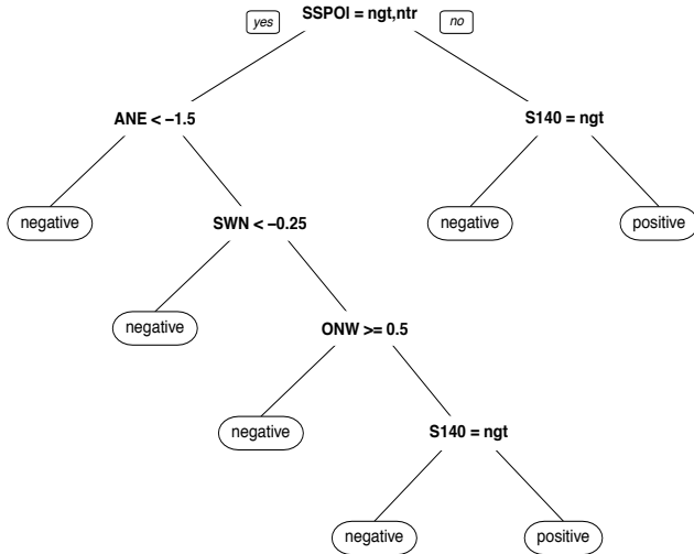
Figure 3: Best Tree trained with CART for polarity classification on the Sanders dataset
